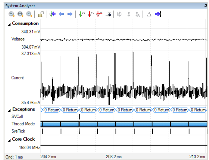
System Analyzer shows power measurement data synchronized to events, interrupts, and variable changes.
